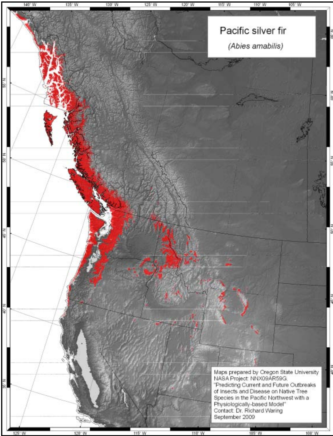
Model predicted range of Pacific silver fir using long term climate data
