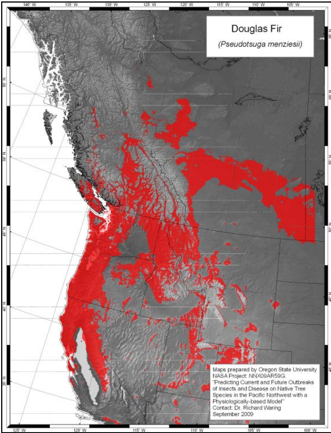
Model predicted range of Douglas-fir using long term climate data
