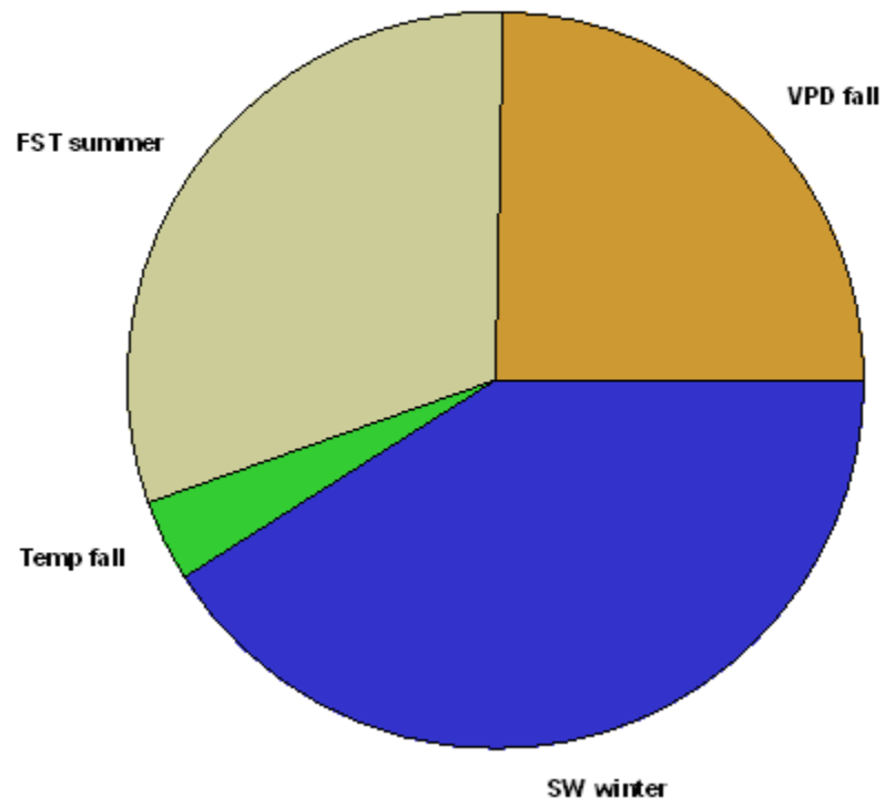
Pie chart showing relative effects of most influential model variables for the species
